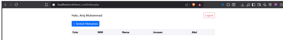
Gambar 5. Tampilan index.php
