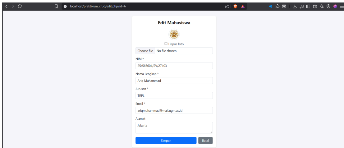
Gambar 9. Tampilan edit.php
